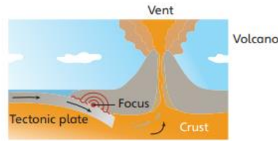
Earthquakes occur when plates jolt forward after getting stuck
