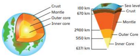
Layers of the Earth
